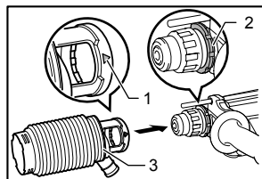
1. \Delta symbol 2. Grooves 3. Dust cup
